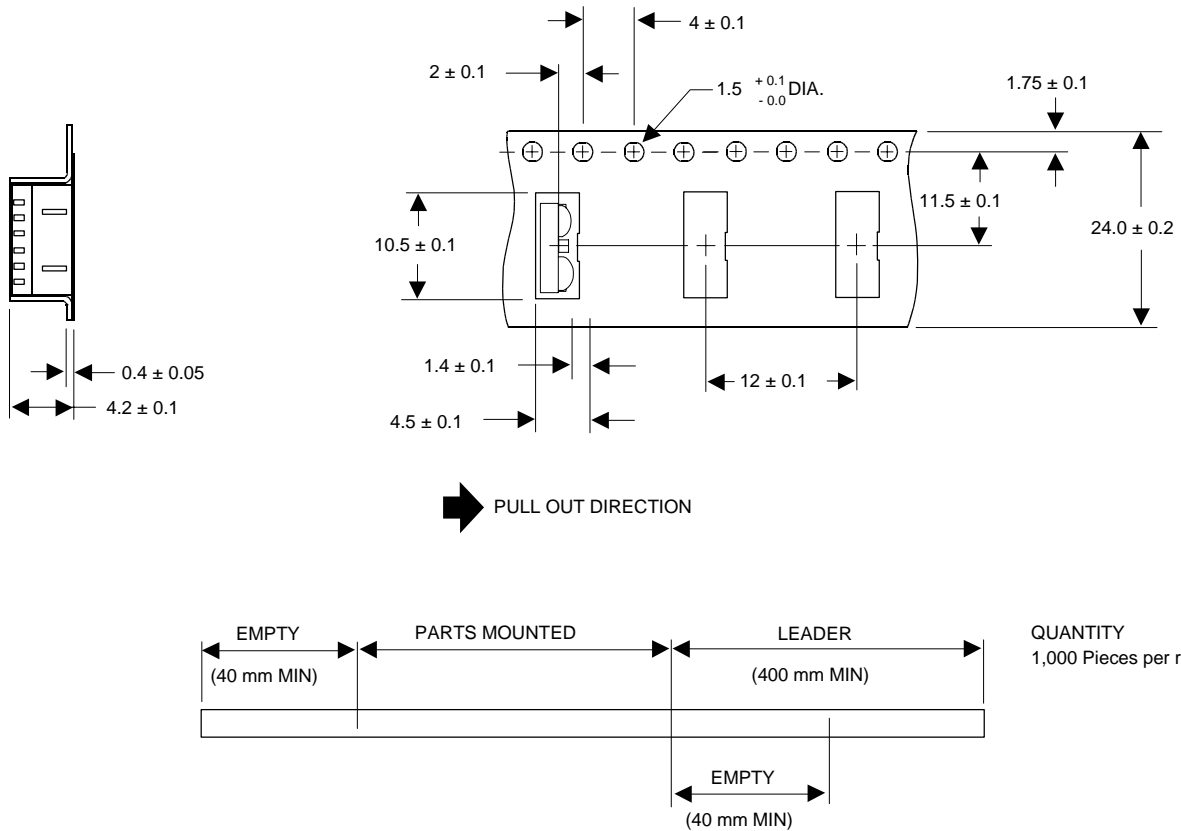
Figure 8. ZHX1010 Tape Dimensions and Configuration (Unit: mm)
