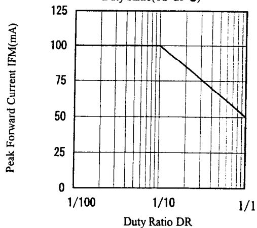
Peak Forward Current vs. Duty Ratio ( T_a=25^\circ\text{C} )
