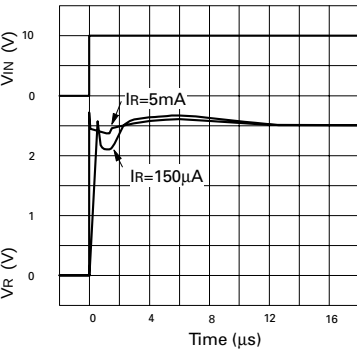
Transient Response - Repetitive Test
