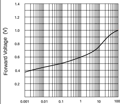
Forward Characteristics
