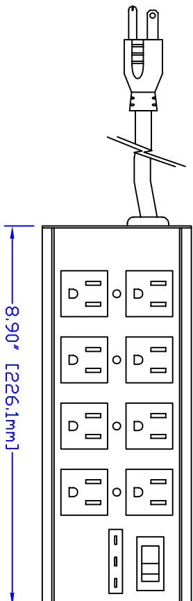
TOP VIEW
