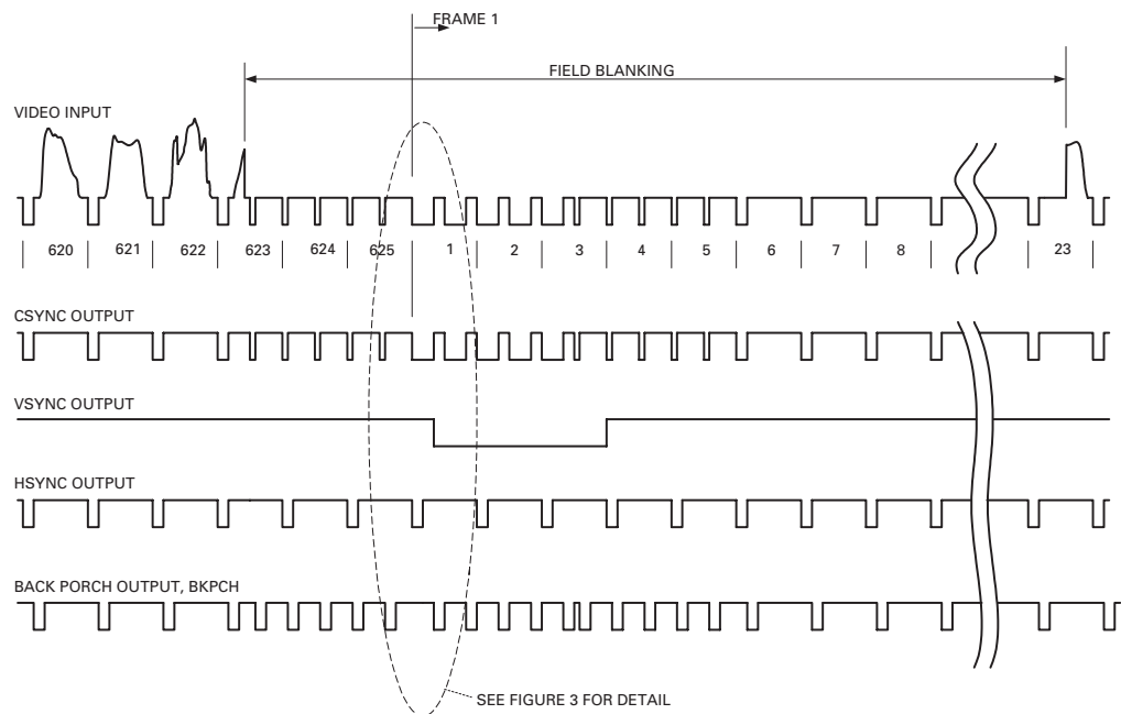
Figure 1: PAL 625 TIMING DIAGRAM
