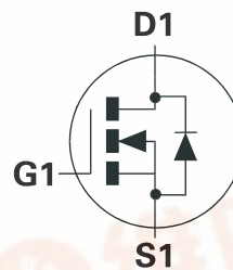
Q1 = N-CHANNEL
