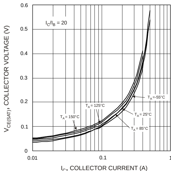
Fig. 6 V_{CE(SAT)} vs. I_C @ I_C/I_B = 20
