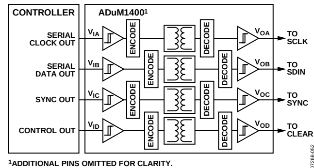
Figure 58. Isolated Interface
