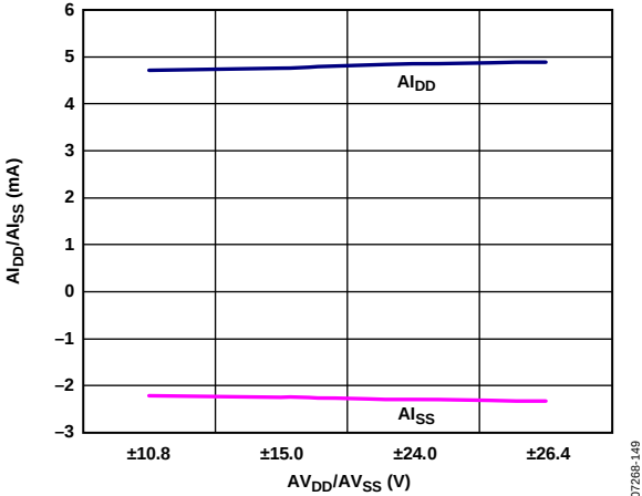
Figure 49. A_{DD}/A_{SS} vs. AV_{DD}/AV_{SS} , V_{OUT} = 0 V
