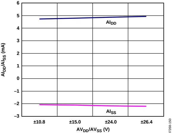
Figure 50. A_{DD}/A_{SS} vs. AV_{DD}/AV_{SS} , I_{OUT} = 0 mA
