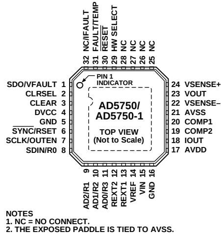
Figure 4. Pin Configuration
