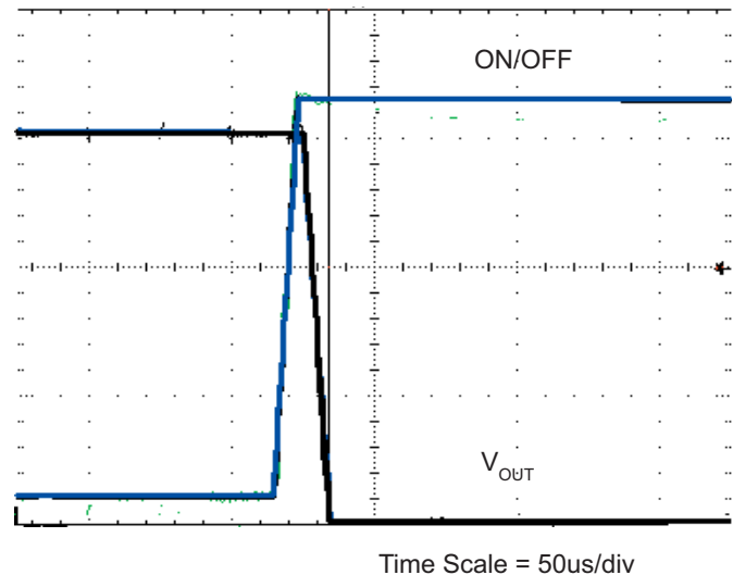
Primary Off Time (Primary Remote to V_{out} )
