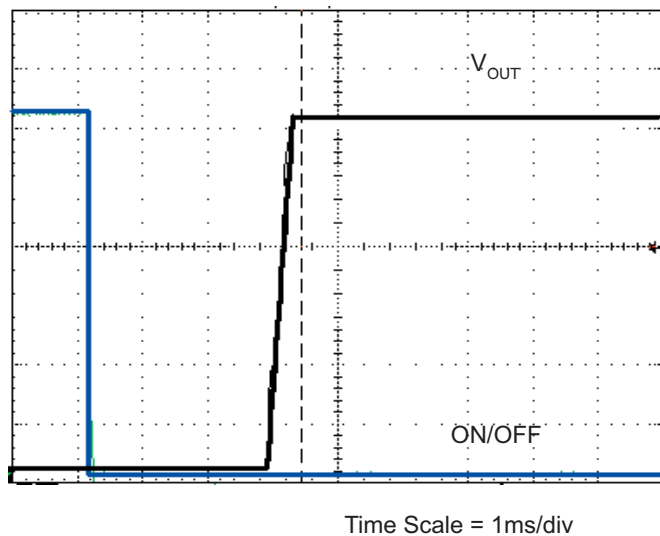
Primary On Time (Primary Remote to V_{out} )
