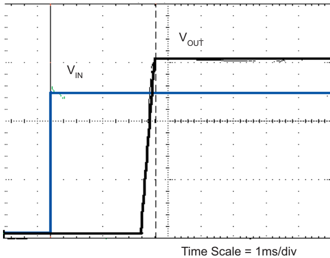
Primary On Time (Primary Remote to V_{out} )
