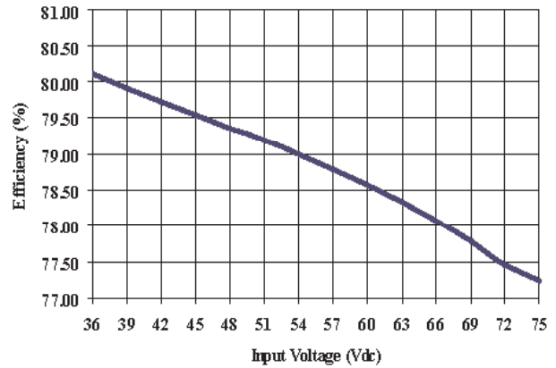
Efficiency vs. Input Voltage @ T_A = +25^\circ\text{C} ; I_o = 40\text{A}
