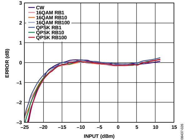
Figure 26. Error from CW Linear Reference vs. Input with Various LTE Reverse Link Waveforms at 2600 MHz, C_{FLTR} = 12 nF, C_{OUT} = \text{Open}
