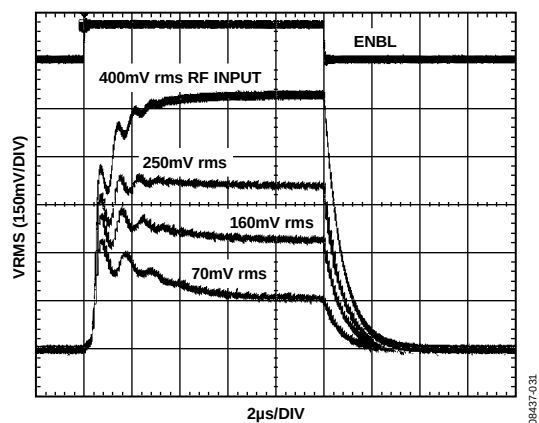
Figure 31. Output Response to Enable Gating at Various RF Input Levels, 3.0 V Supply, 900 MHz Frequency, C_{FLTR} = Open, C_{OUT} = Open, R_{OUT} = Open
