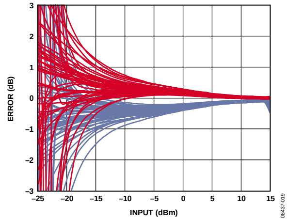
Figure 19. Output Delta from +25°C Output Voltage for 50 Devices at -40°C and +85°C, 2600 MHz Frequency
