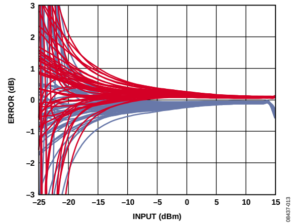
Figure 13. Output Delta from +25°C Output Voltage for 50 Devices at -40°C and +85°C, 450 MHz Frequency
