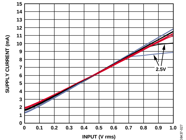
Figure 27. Supply Current vs. Input Level, 2.5 V, 3.0 V, and 3.3 V Supplies, 900 MHz Frequency, at -40^{\circ}\text{C} , +25^{\circ}\text{C} , and +85^{\circ}\text{C}
