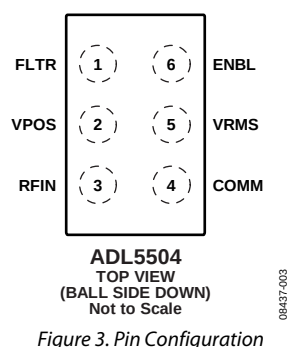
Figure 3. Pin Configuration
