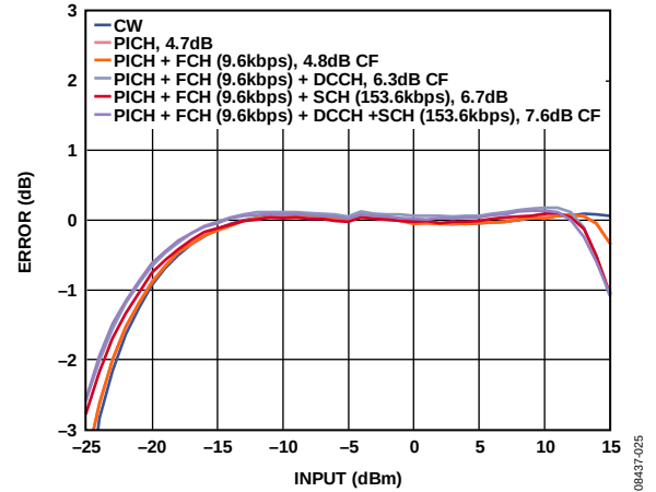
Figure 25. Error from CW Linear Reference vs. Input with Various CDMA2000 Reverse Link Waveforms at 1900 MHz, C_{FLTR} = 12 nF, C_{OUT} = \text{Open}
