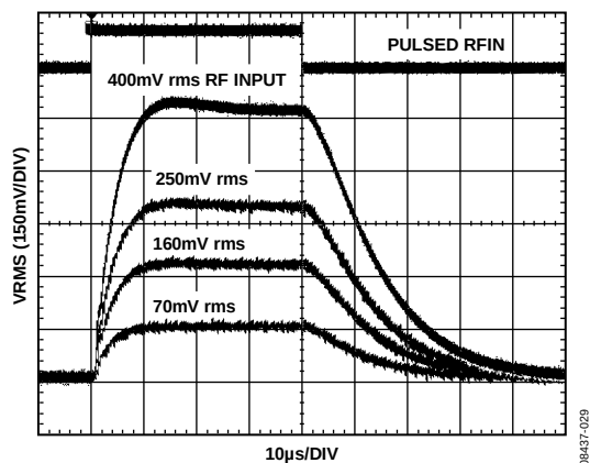
Figure 29. Output Response to Various RF Input Pulse Levels, 3.0 V Supply, 900 MHz Frequency, C_{FLTR} = 10 nF, C_{OUT} = Open, R_{OUT} = Open
