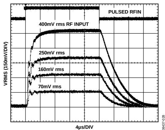
Figure 28. Output Response to Various RF Input Pulse Levels, 3.0 V Supply, 900 MHz Frequency, C_{FLTR} = Open, C_{OUT} = Open, R_{OUT} = Open
