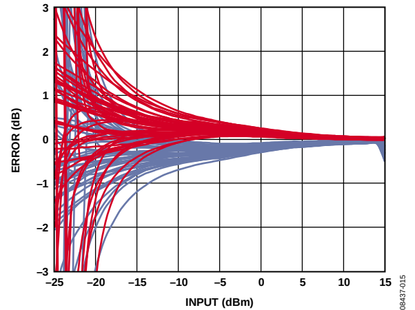
Figure 15. Output Delta from +25°C Output Voltage for 50 Devices at -40°C and +85°C, 1900 MHz Frequency
