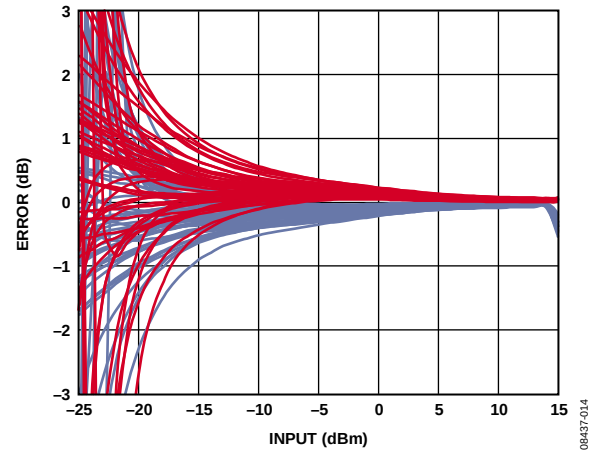
Figure 14. Output Delta from +25°C Output Voltage for 50 Devices at -40°C and +85°C, 900 MHz Frequency
