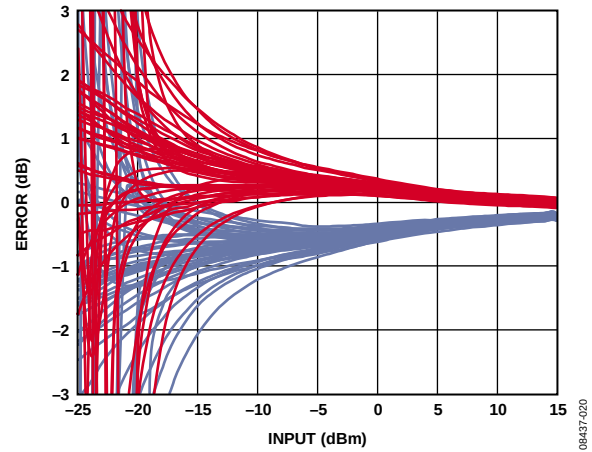
Figure 20. Output Delta from +25°C Output Voltage for 50 Devices at -40°C and +85°C, 3500 MHz Frequency
