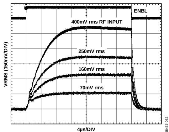
Figure 32. Output Response to Enable Gating at Various RF Input Levels, 3.0 V Supply, 900 MHz Frequency, C_{FLTR} = 10 nF, C_{OUT} = Open, R_{OUT} = Open
