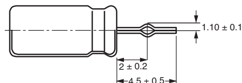
10 ≤ Ø D ≤ 18 leads shortened and formed MALREKE06... (S = 5/7.5 mm)
