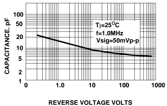
Fig. 6-TYPICAL JUNCTION CAPACITANCE
