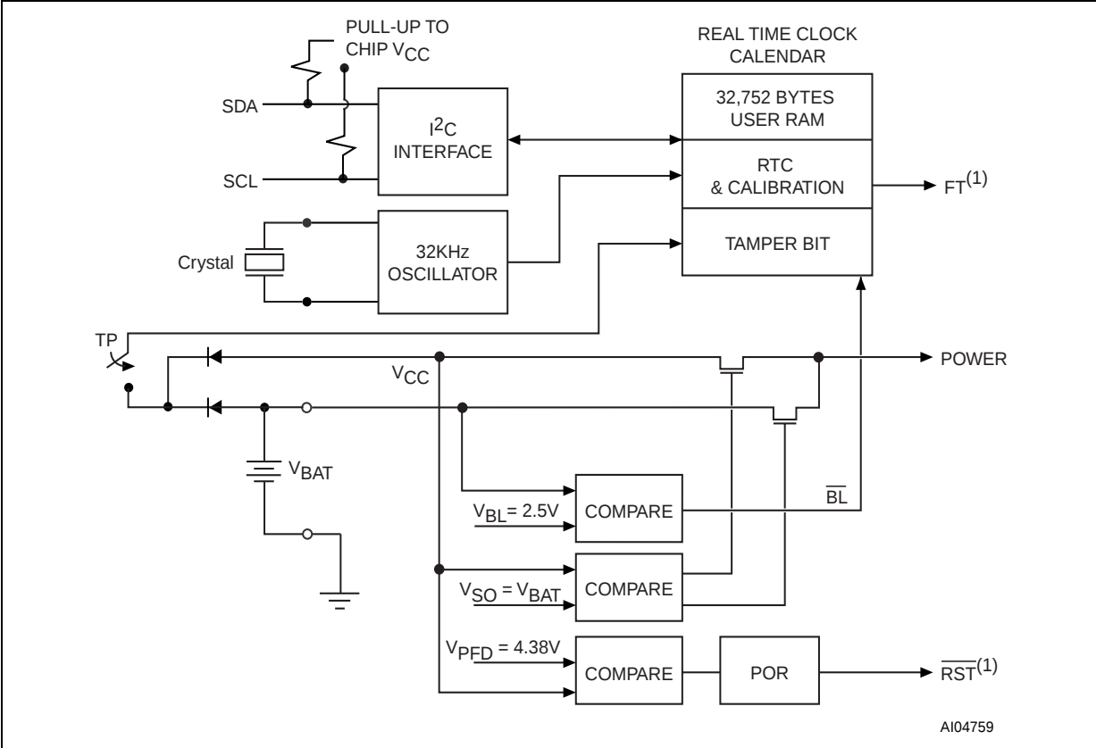
Figure 6. Block Diagram
