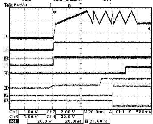
FIGURE 10. START-UP SEQUENCE
