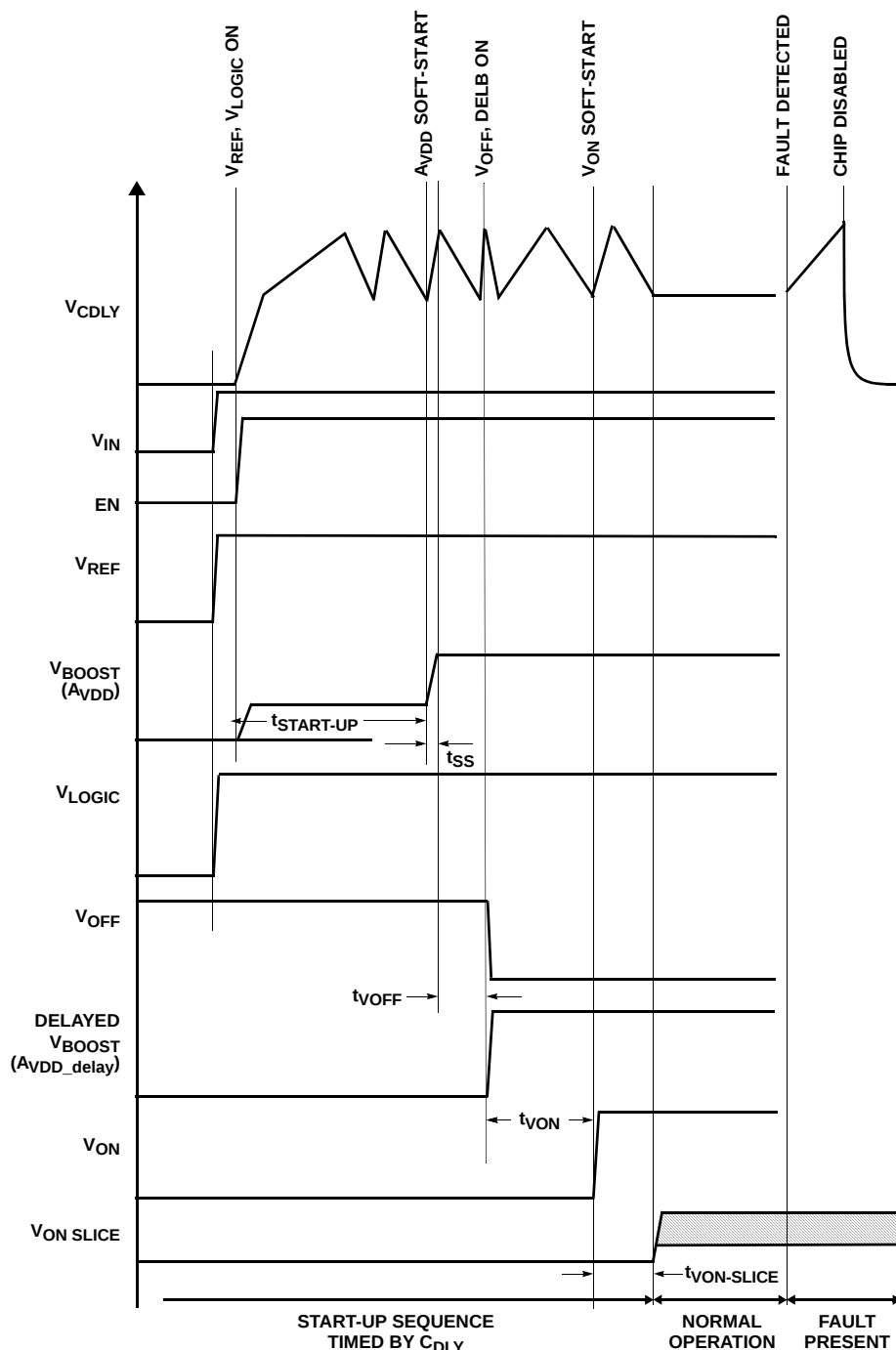
FIGURE 15. START-UP SEQUENCE
