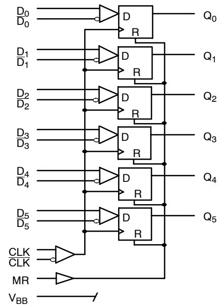
Figure 2. Logic Diagram
