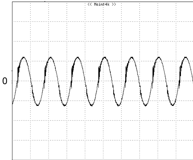
Figure 11: Input Terminal Ripple Current, i_c , at full rated output current and nominal input voltage with 12\mu\text{H} source impedance and 33\mu\text{F} electrolytic capacitor (500 mA/div, 2μs/div)
