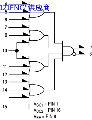
Figure 1. Logic Diagram
