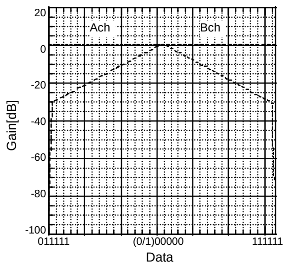
Balance Control
