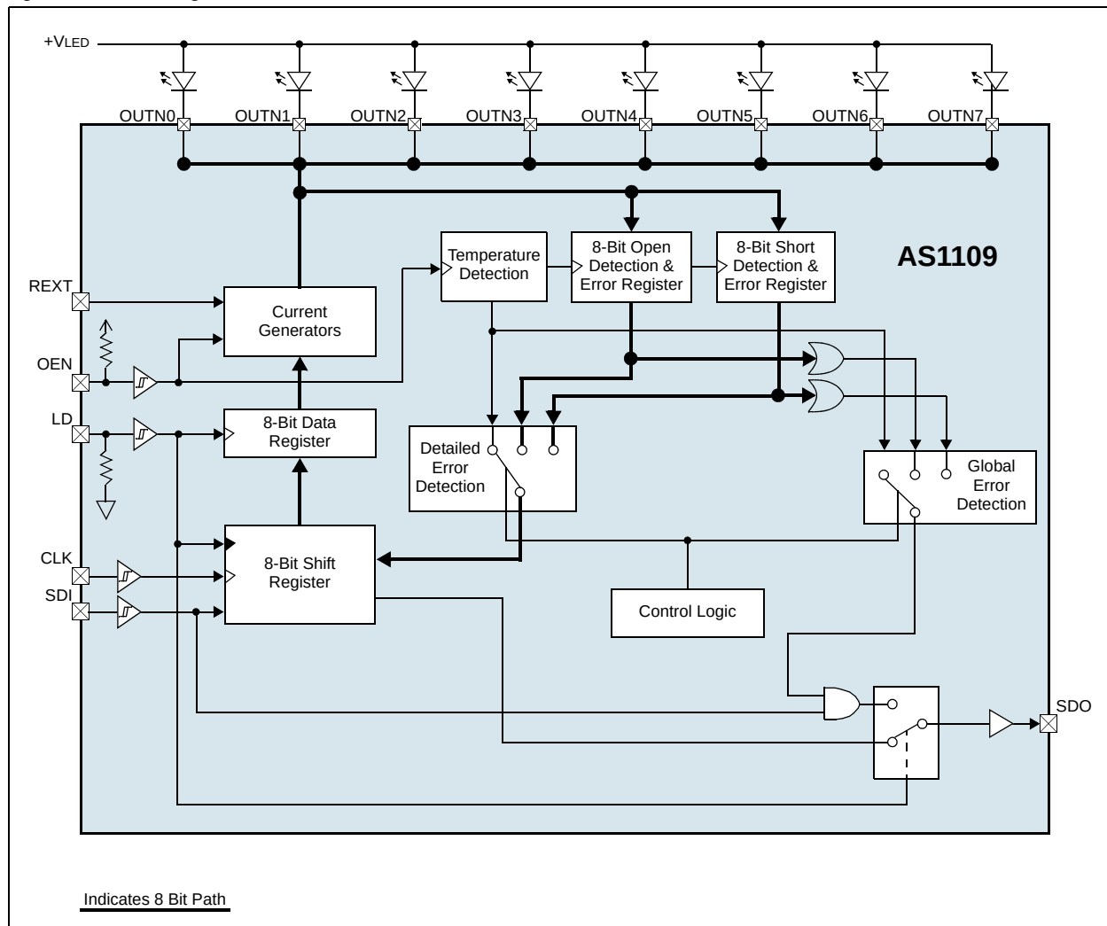
Figure 9. Block Diagram
