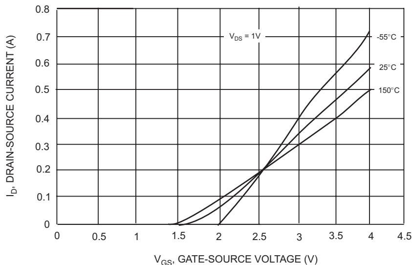
Fig. 2 Transfer Characteristics
