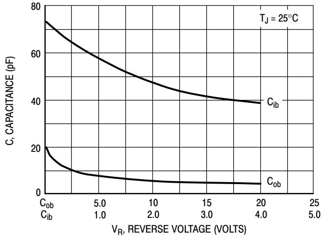
Figure 9. Capacitance
