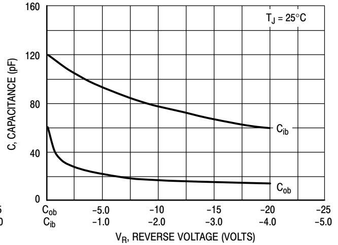
Figure 10. Capacitance
