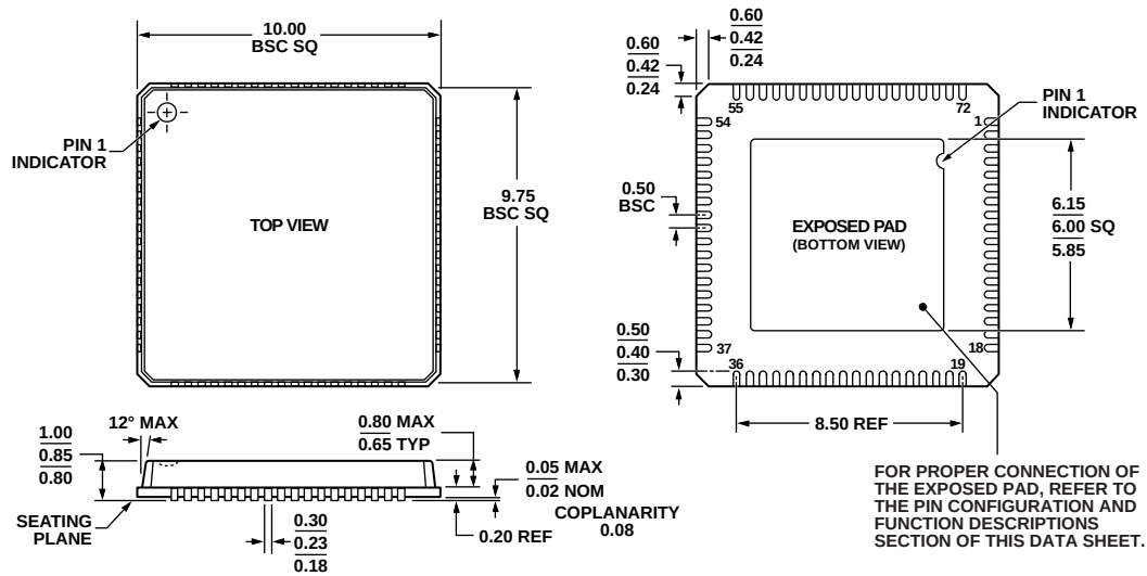
Figure 86. 72-Lead Lead Frame Chip Scale Package [LFCSP_VQ] 10 mm × 10 mm Body, Very Thin Quad (CP-72-7) Dimensions shown in millimeters
