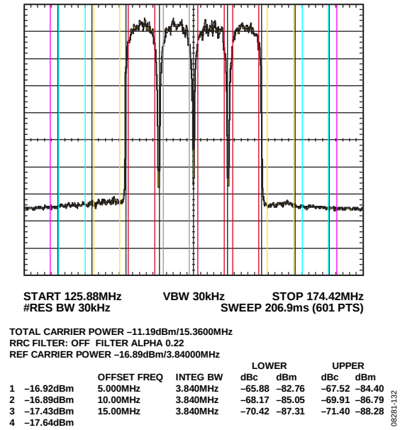
Figure 35. 1-Carrier W-CDMA ACLR Performance, IF = ~150 MHz
