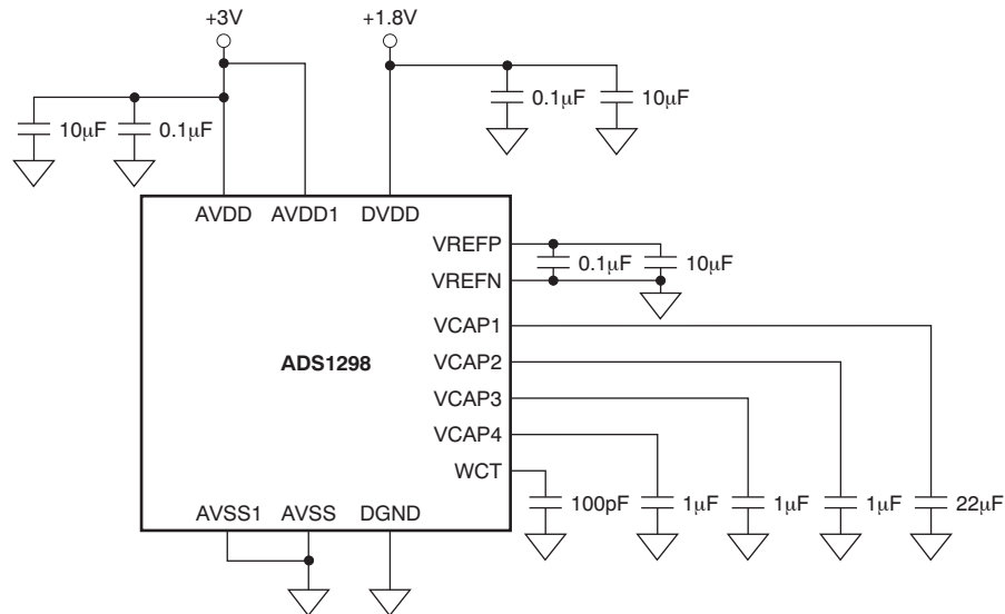
Figure 59. Single-Supply Operation
