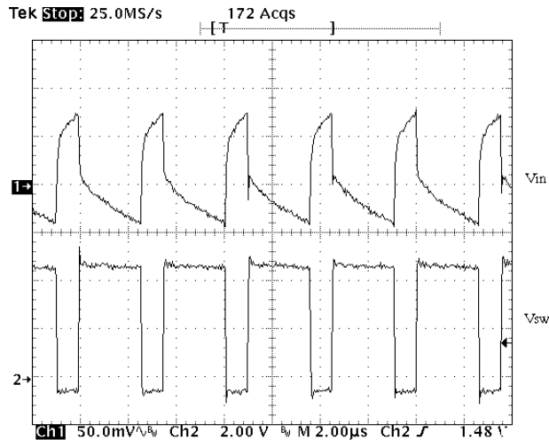
Figure 18. Input Voltage Ripple in a Buck Converter
