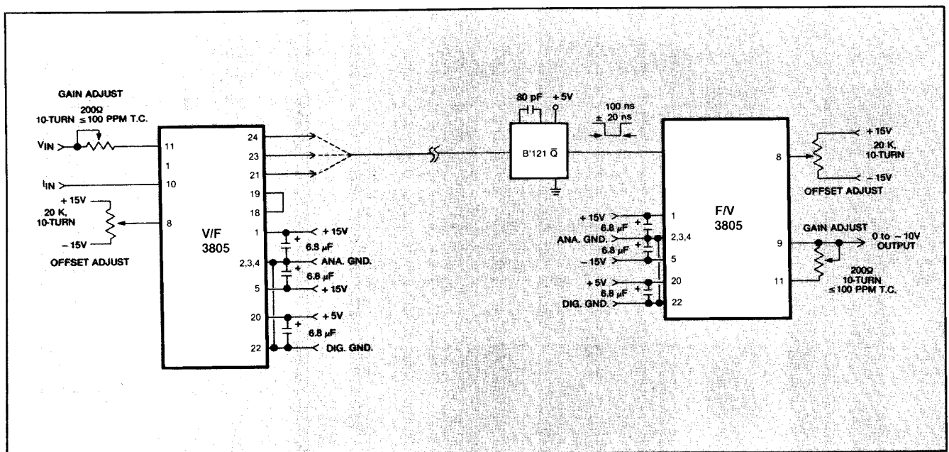
Figure 5. 5 MHz Analog Data Link.
