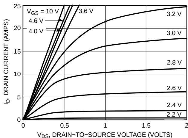
Figure 2. On-Region Characteristics
