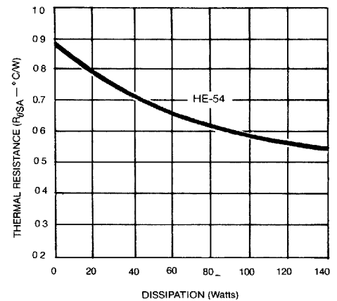
Typical Heat Sink Characteristics
