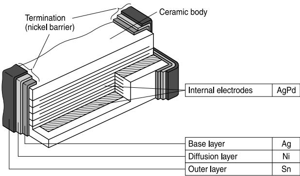
Multilayer CTVS: Structure of nickel barrier termination
