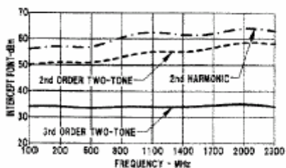
Intercept Point
