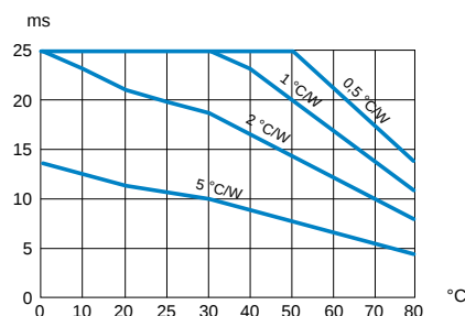
Thermal curves
