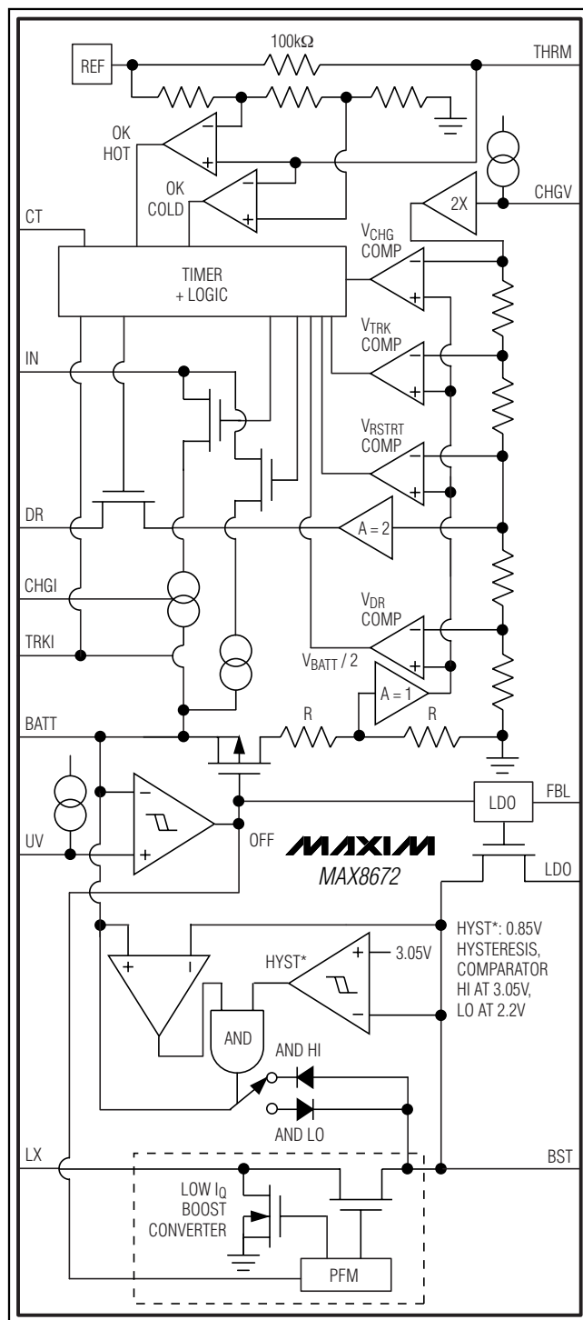
Figure 1. MAX8672 Functional Block Diagram
