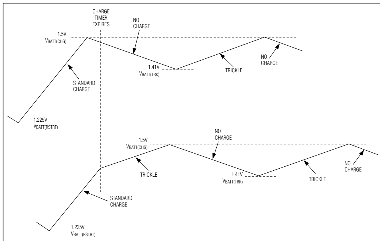
Figure 2. Typical Charge-Current Profiles for 1-Cell Battery
