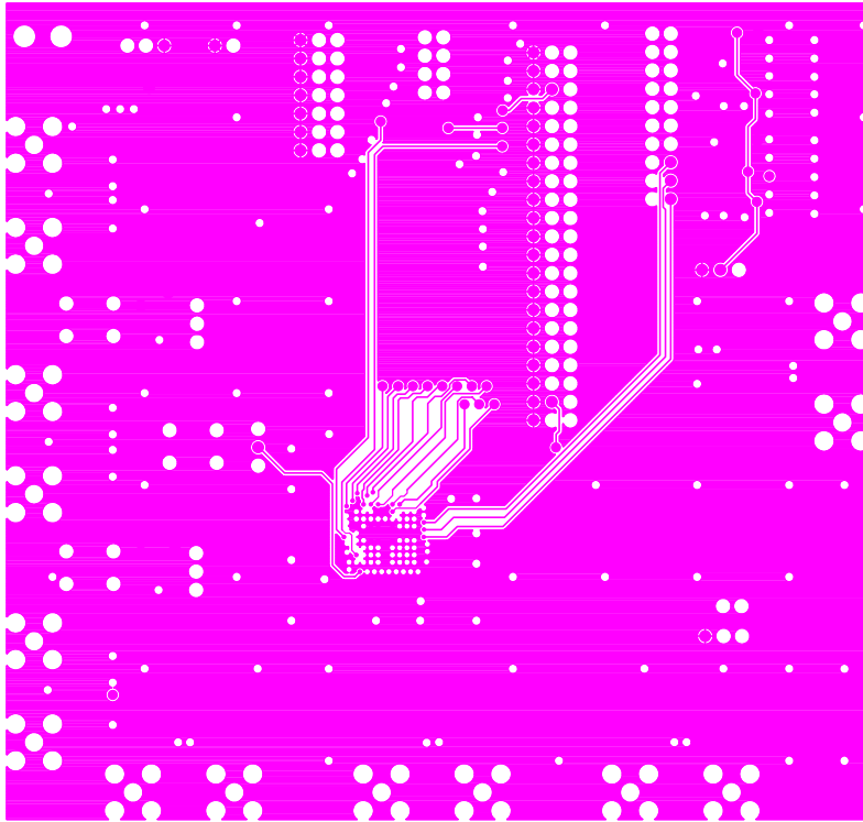
Figure 9. Si5364-EVB—Layer 6, VDD 3.3
