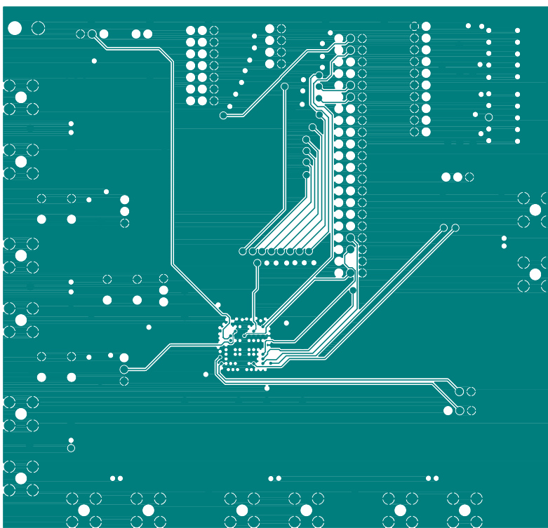
Figure 8. Si5364-EVB—Layer 5, GND
