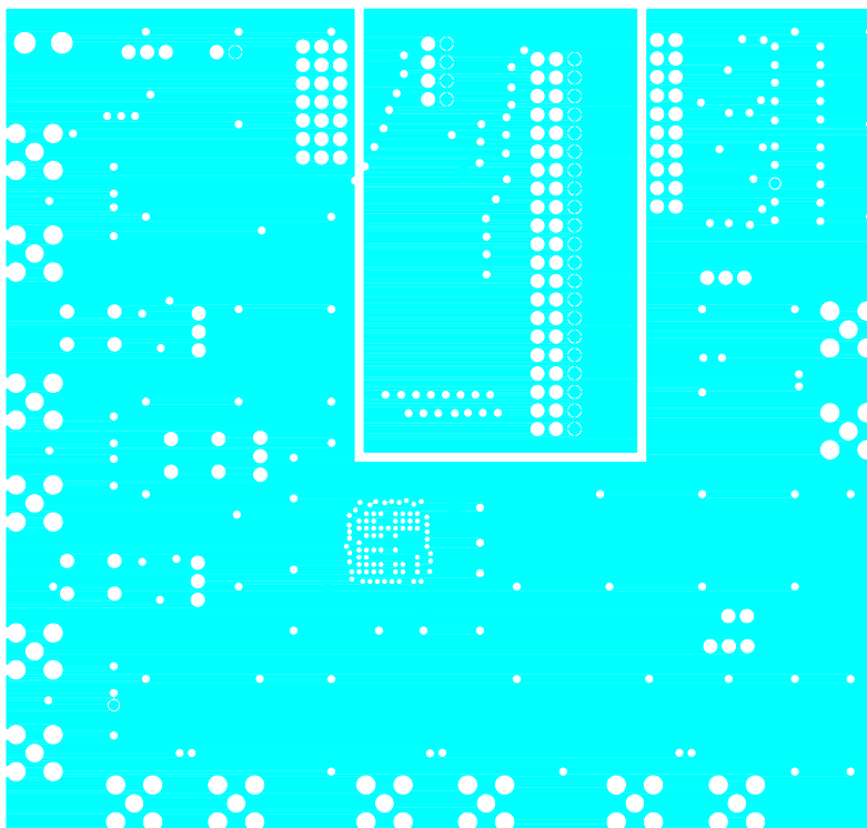
Figure 7. Si5364-EVB—Layer 4, VDD 2.5
