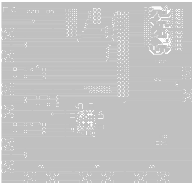
Figure 11. Si5364-EVB—Layer 8, Bottom
