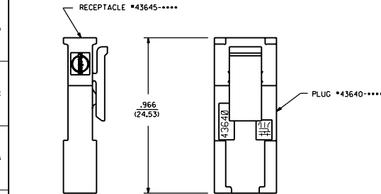
MATED MICRO-FIT CONNECTOR
