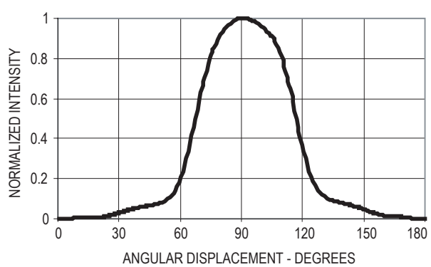
Figure 9. Radiation pattern for HLMP-CY46/47
