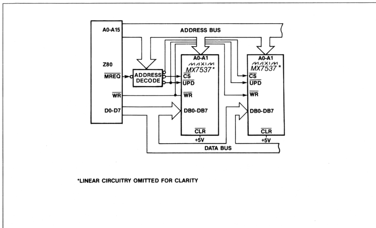
Figure 12. Expanded MX7537 System
