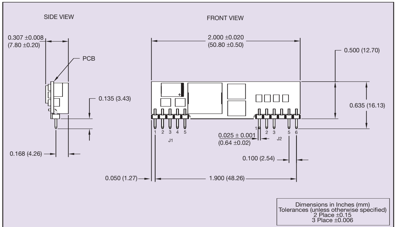
Figure 34: Mechanical Drawing
