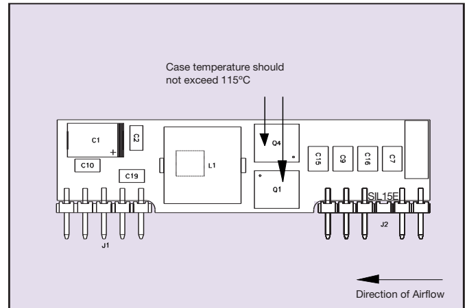
Figure 36: Thermal Reference Points
