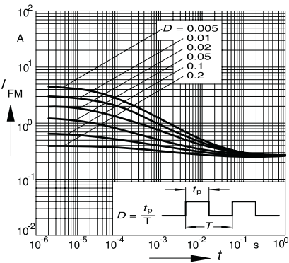
Figure 2. Peak forward current I FM = f (t p )
