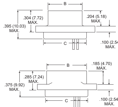
MDB Glass-filled Diallyl Phthalate Plastic Insulator
