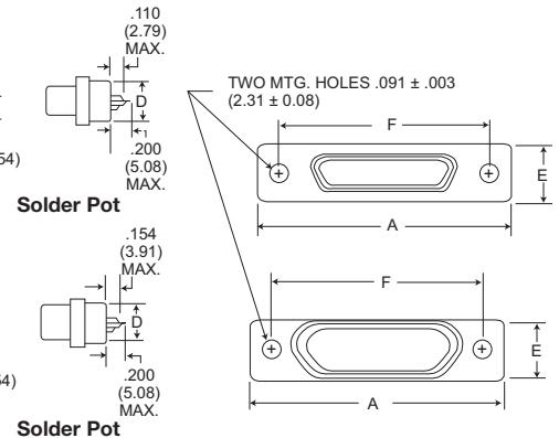
MDVB Glass-filled Polyester Plastic Insulator
