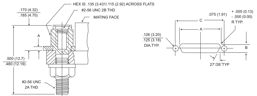
Plug and Receptacle Dimensions
