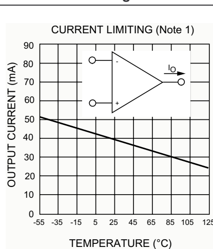
Figure 9. Current limiting
