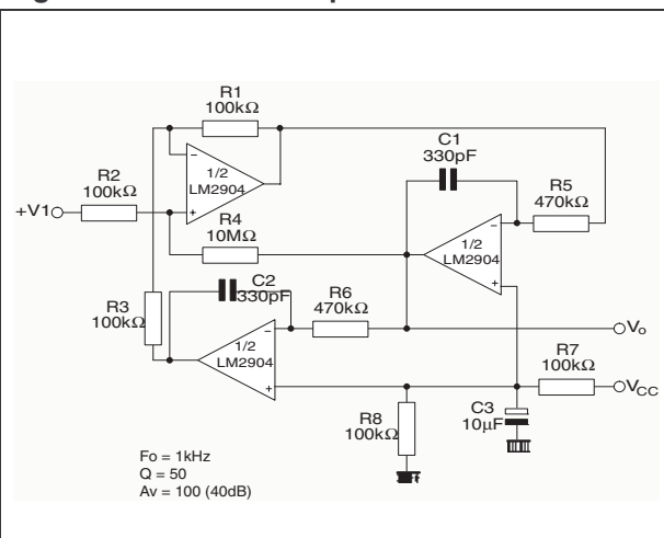
Figure 25. Active bandpass filter
