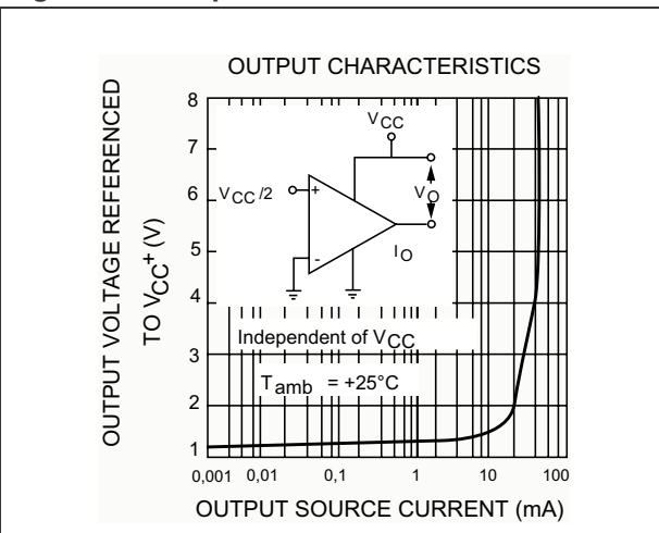
Figure 7. Output characteristics
