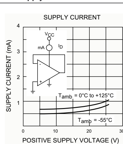
Figure 11. Supply current
