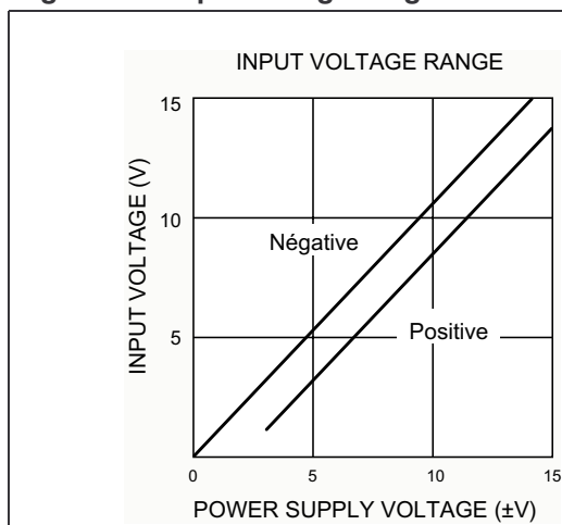
Figure 10. Input voltage range
