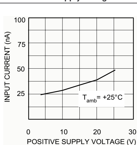
Figure 13. Positive supply voltage
