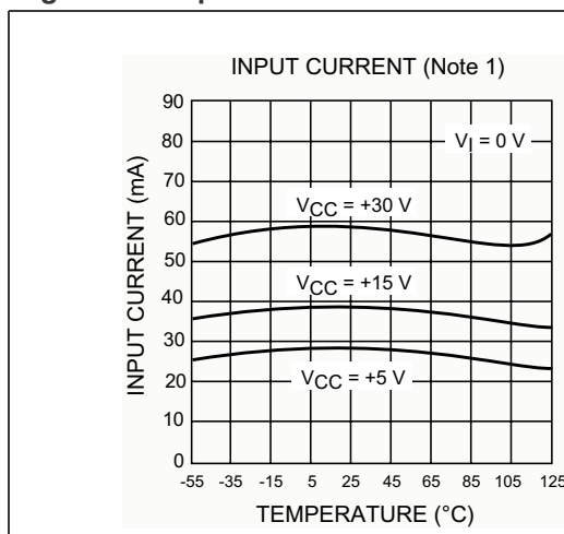
Figure 8. Input current
