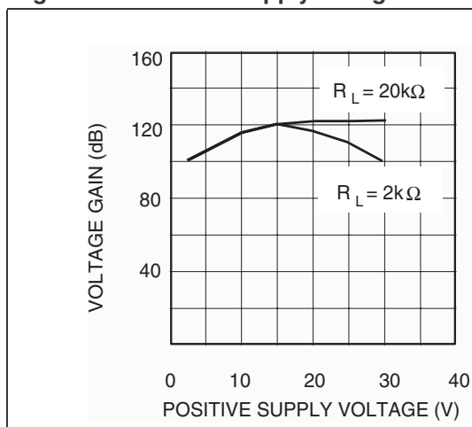
Figure 12. Positive supply voltage
