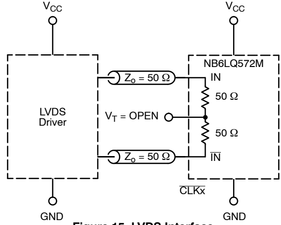
Figure 15. LVDS Interface
