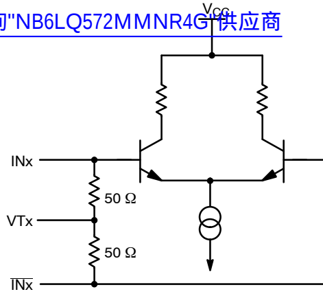
Figure 6. Input Structure
