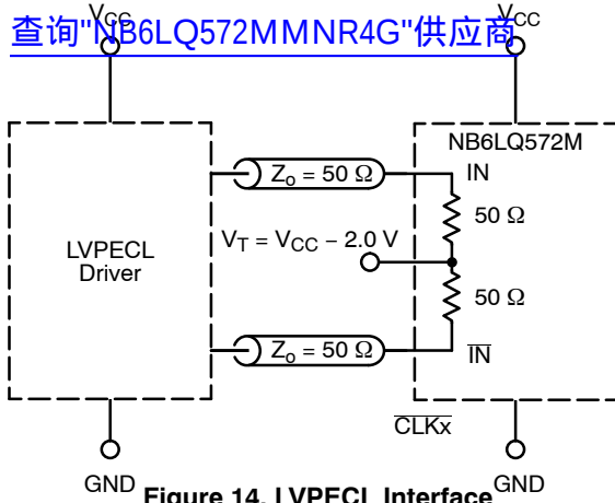
Figure 14. LVPECL Interface
