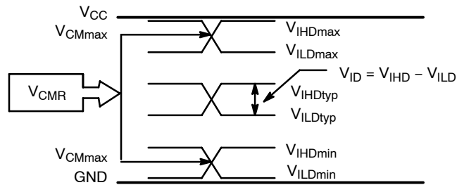
Figure 18. V_{CM} Diagram
