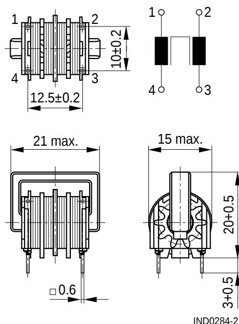
Vertical version (B82731M)
