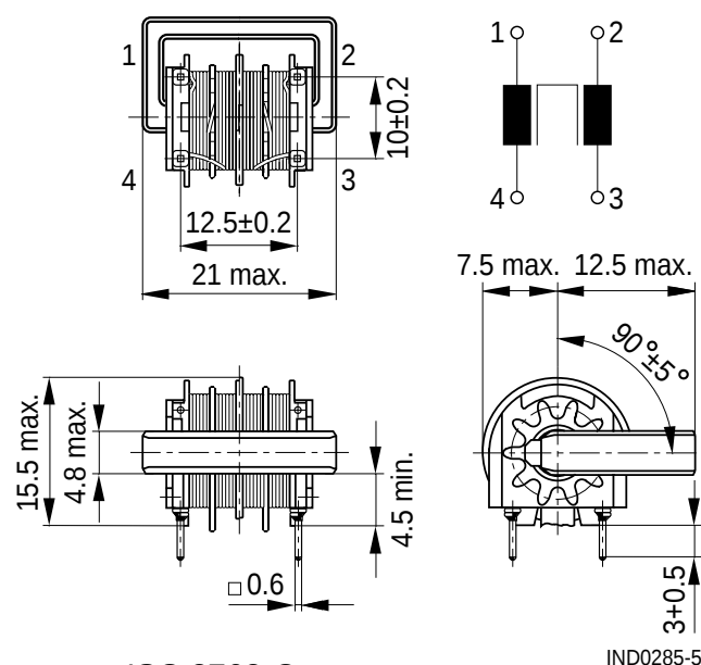
Horizontal version (B82731H)
