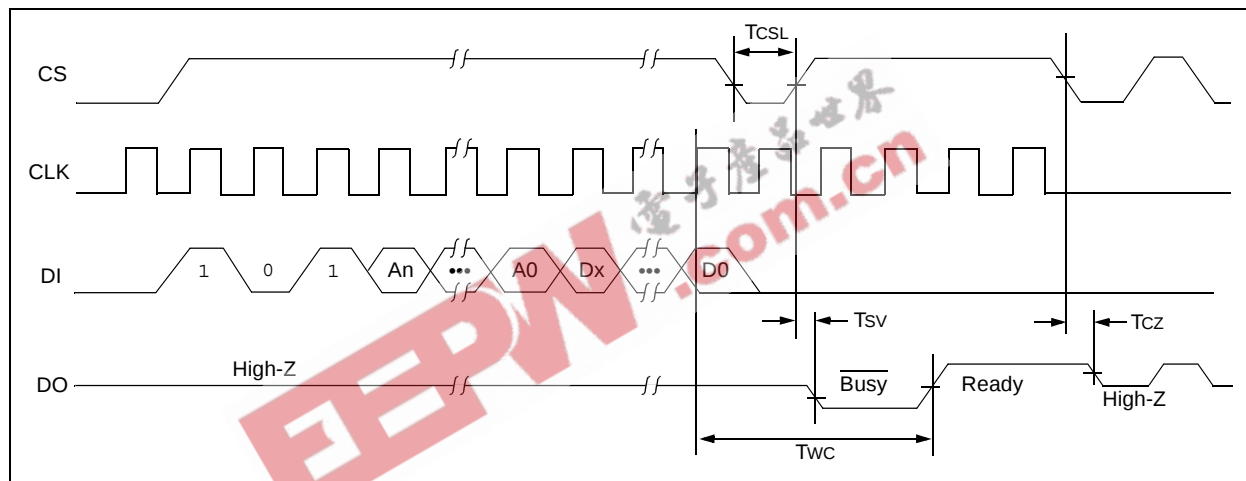
FIGURE 2-6: WRITE TIMINGS
