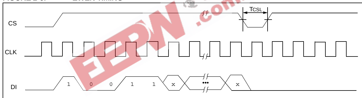
FIGURE 2-6: EWEN TIMING
