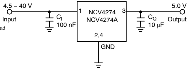
Figure 3. Application Circuit
