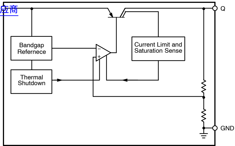
Figure 1. Block Diagram
