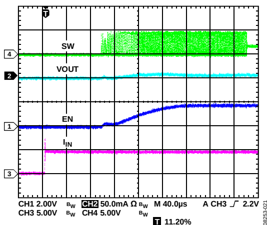
Figure 6. Buck1 Startup, VOUT1 = 3.3 V, I OUT1 = 10 mA
