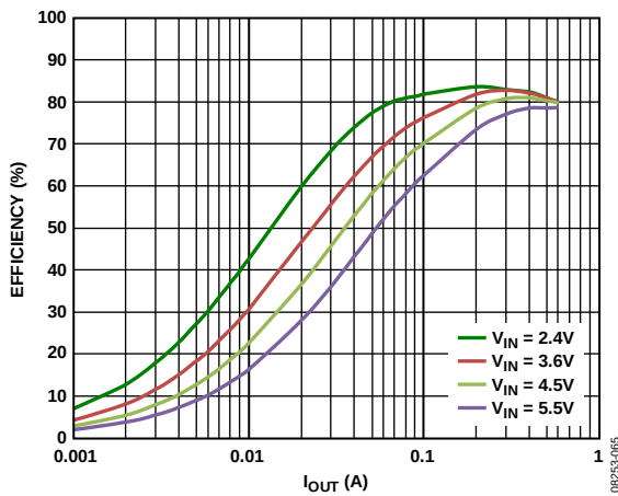
Figure 18. Buck1 Efficiency vs. Load Current, Across Input Voltage, VOUT1 = 0.8 V, PWM Mode
