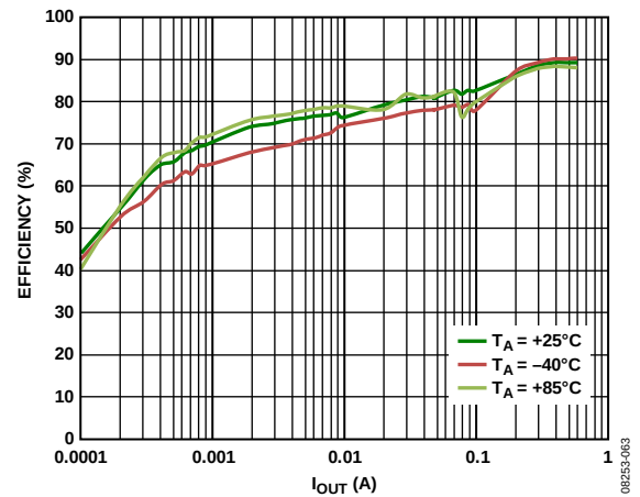
Figure 20. Buck2 Efficiency vs. Load Current, Across Temperature, VOUT2 = 1.8 V, Auto Mode
