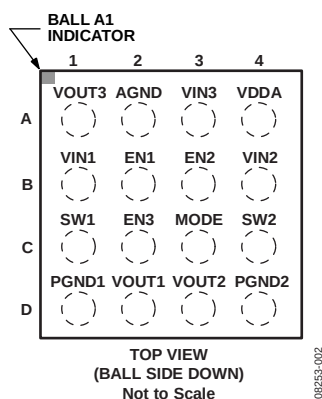
Figure 3. Pin Configuration
