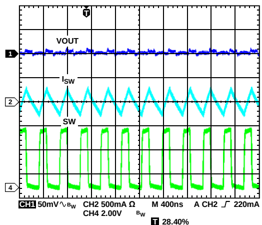
Figure 25. Typical Waveforms, V_{OUT2} = 1.8\text{ V} , I_{OUT2} = 30\text{ mA} , PWM Mode
