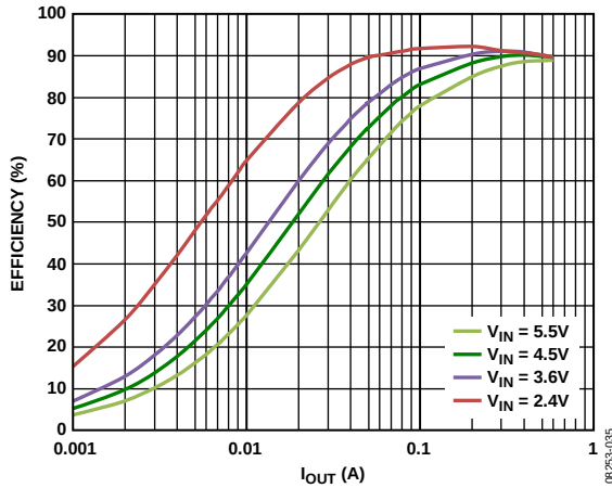
Figure 16. Buck2 Efficiency vs. Load Current, Across Input Voltage, VOUT2 = 1.8 V, PWM Mode
