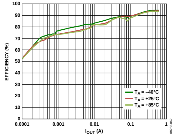
Figure 19. Buck1 Efficiency vs. Load Current, Across Temperature, VOUT1 = 3.3 V, Auto Mode
