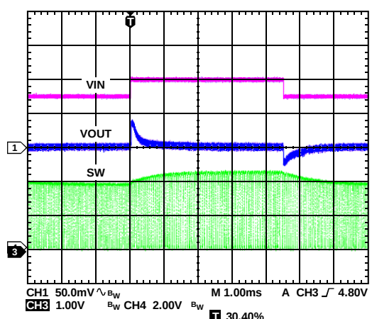
Figure 27. Buck2 Response to Line Transient, V_{IN} = 4.5\text{ V} to 5.0\text{ V} , V_{OUT2} = 1.8\text{ V} , PWM Mode
