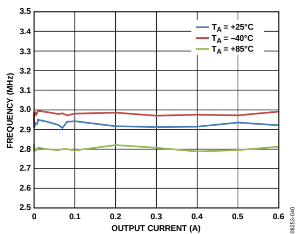
Figure 21. Buck2 Switching Frequency vs. Output Current, Across Temperature, VOUT2 = 1.8 V, PWM Mode
