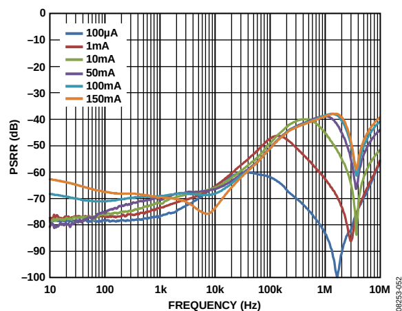
Figure 47. LDO PSRR Across Output Load, V_{IN3} = 5.0\text{ V} , V_{OUT3} = 3.0\text{ V}
