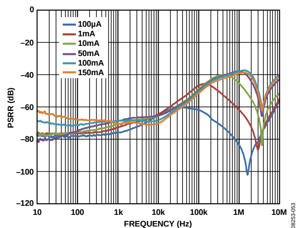
Figure 46. LDO PSRR Across Output Load, V_{IN3} = 5.0\text{ V} , V_{OUT3} = 2.8\text{ V}
