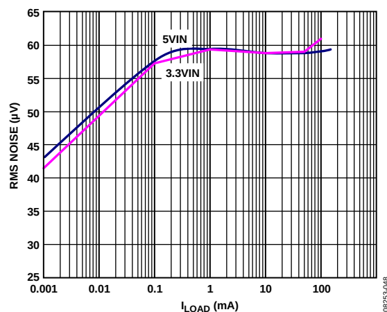
Figure 43. LDO Output Noise vs. Load Current, Across Input Voltage, V_{OUT3} = 3.0 V
