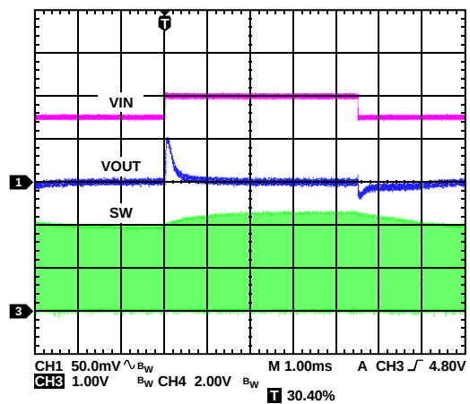
Figure 26. Buck1 Response to Line Transient, Input Voltage from 4.5\text{ V} to 5.0\text{ V} , V_{OUT1} = 3.3\text{ V} , PWM Mode
