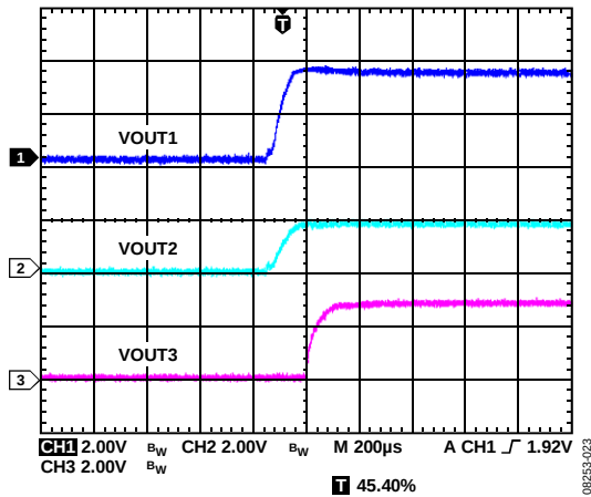
Figure 4. 3-Channel Start-Up Waveforms, VIN3 Cascaded from VOUT1
