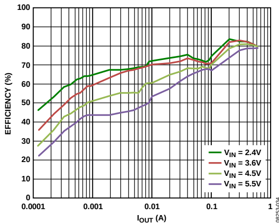
Figure 17. Buck1 Efficiency vs. Load Current, Across Input Voltage, VOUT1 = 0.8 V, Auto Mode
