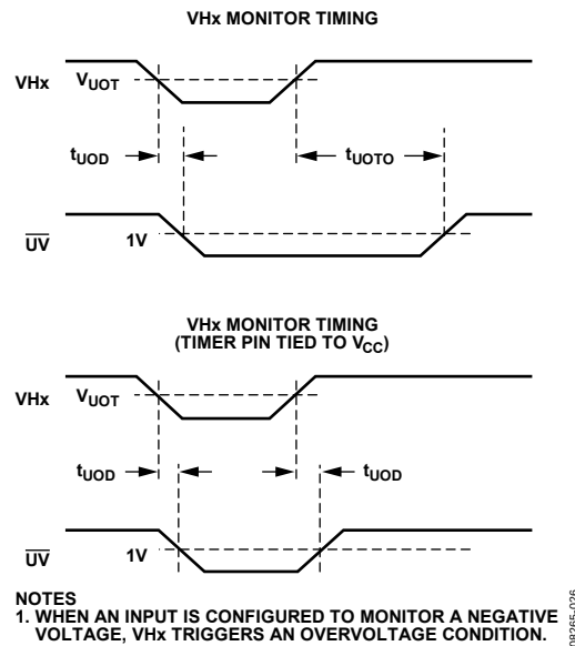
Figure 21. VHx Positive Voltage Monitoring Timing Diagrams
