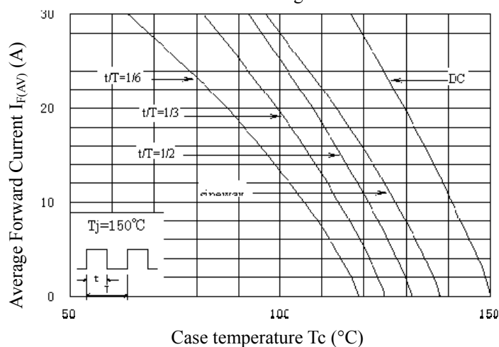
Current Derating
