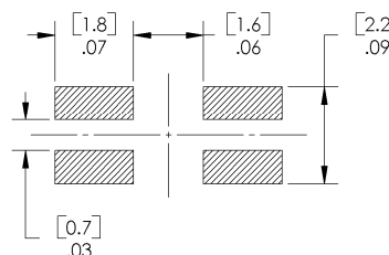
SOLDERING PATTERN
