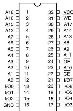
TSOP Top View
